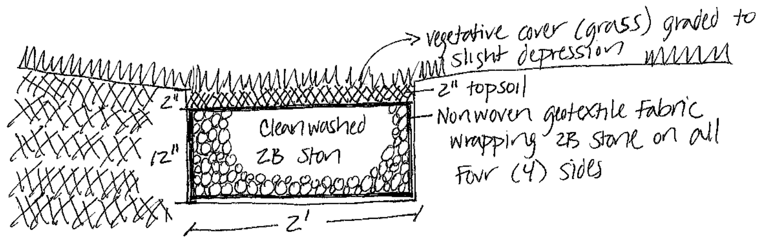
INFILTRATION TRENCH DETAIL
