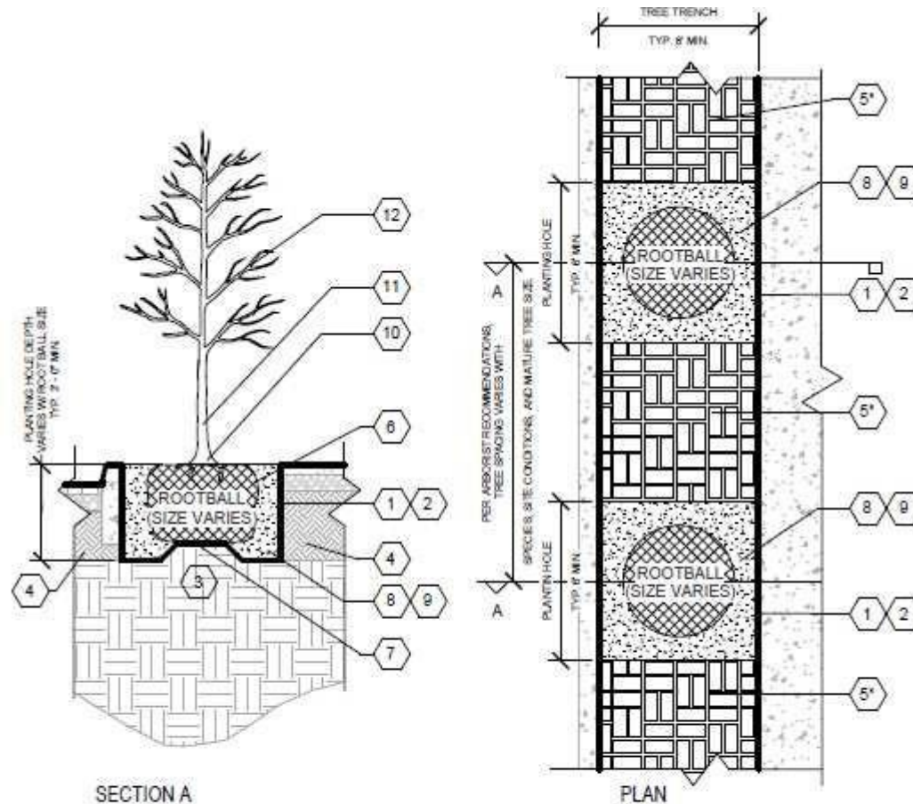
Figure C.7. Street Tree Trench with Engineered Soils
