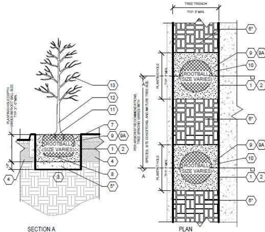
Figure C.6. Street Tree Trench with Structural Soils
